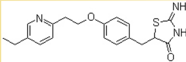
Molecular Structure
